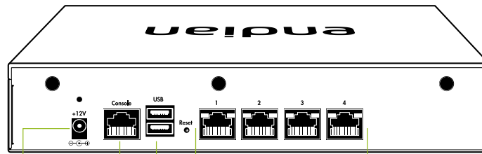
Power Supply Serial Console USB Ports Ethernet Ports 10/100/1000 (RJ-45)
